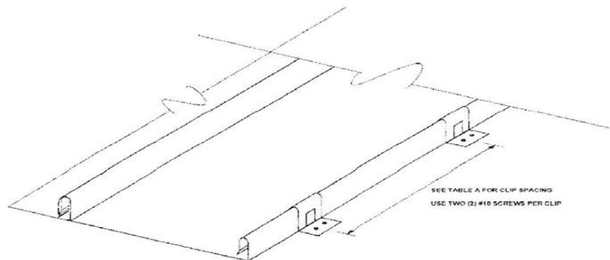
TYPICAL ASSEMBLY ISOMETRIC VIEW
